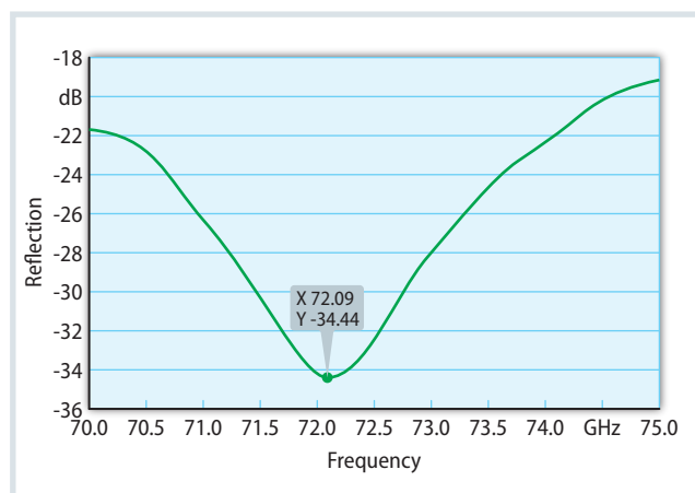
Fig. 6. Frequency response for the reflection measurement on a sheet of Schulablend M/MK 6501 LE: the determined permittivity value is practically equivalent to the result obtained through costly materials testing Source: Rohde & Schwarz; graphic: © Hanser
