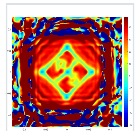
Fig. 4. Visualization of the phase response for the same radome from Figure 1 analyzed with an R&S QAR system: phase angle distortions are clearly visible © Rohde & Schwarz
